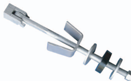
13.02 Quick Acting Cleat Assembly
