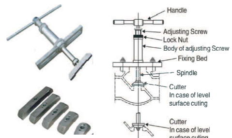
633451 | Valve Seat Cutter 1-4" complete | set
